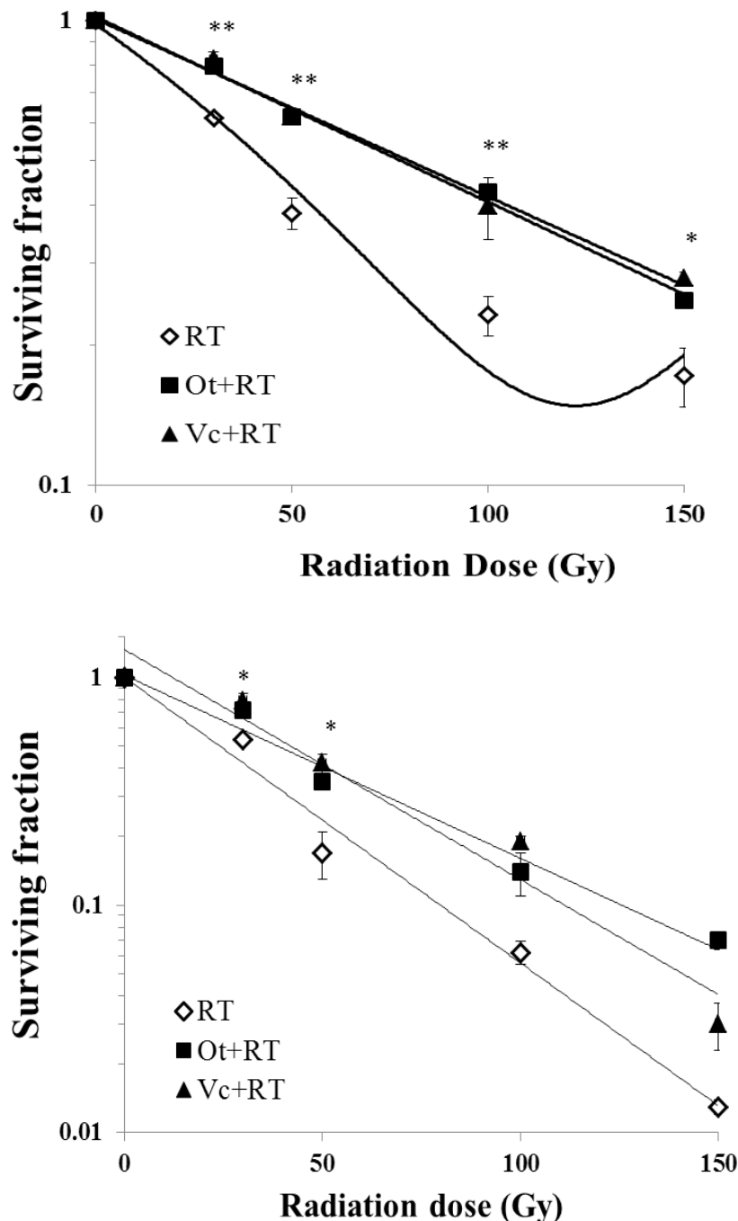
Figure 4: Effect of pretreatment with 200 \mu\text{M} Ot or Vc on clonogenic survival of \gamma -irradiated bacterial cells. (A) Survival of AB1157 E. coli cells. Curve fitting for radiation alone: polynomial ( R^2=0.98 ); Ot+RT and Vc+RT: exponential ( R^2=0.99 ). (B) Survival of MD2130 E. coli cells. All survival data were fitted using exponential function; RT alone ( R^2=0.98 ), Ot+RT ( R^2=0.98 ) and Vc+RT ( R^2=0.95 ). All values represent mean values of surviving fractions \pm SEM of 3 independent experiments normalized to control values and plotted as a function of radiation dose. * p < 0.05 , ** p < 0.01 compared to the irradiated group.
