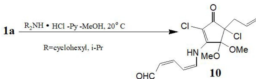
Figure 5: Reaction of chlorocyclopentenone (1a) with hindered amines
