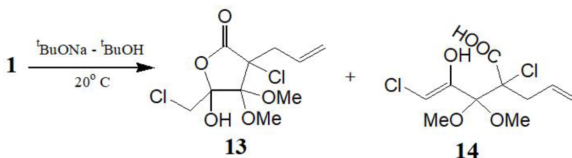
Figure 7: Reaction of chlorocyclopentenone (1) with tert-butyrate anion
