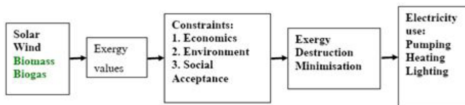
Figure 11: Exergy based optimal energy model [2]
