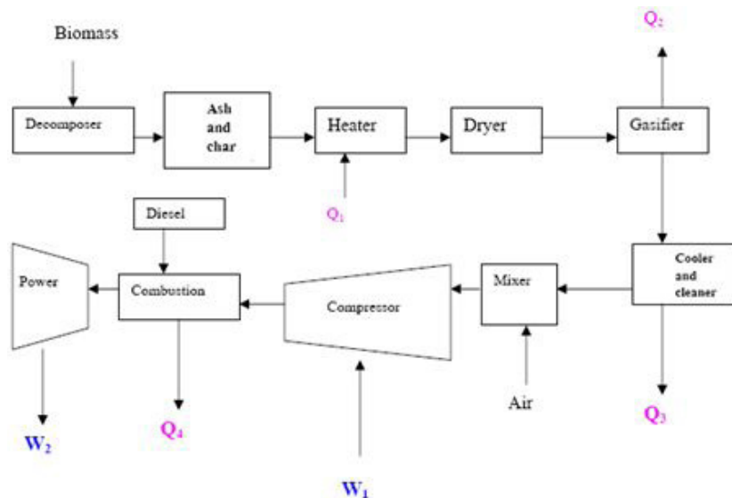
Figure 7: Advanced biomass power with diesel engine [12]
