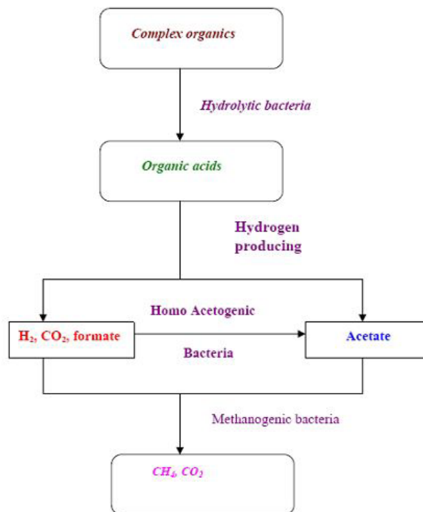
Figure 3: Biogas production process [19]
