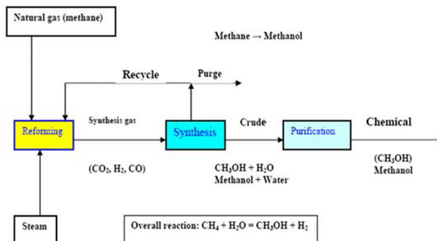
Figure 2: Schematic diagram shows methanol production [12]
