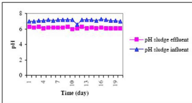
Figure 6: Potential of hydrogen sludge before and after treatment in the digester [12]
