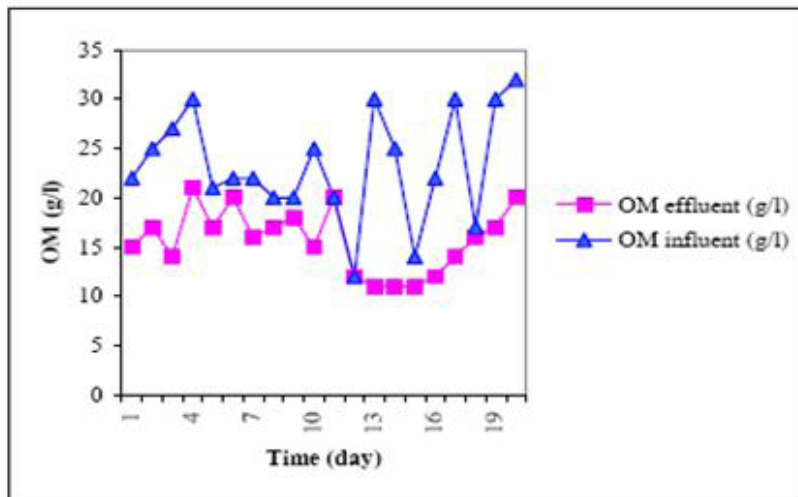
Figure 5: Organic matters before and after treatment in digester [12]
