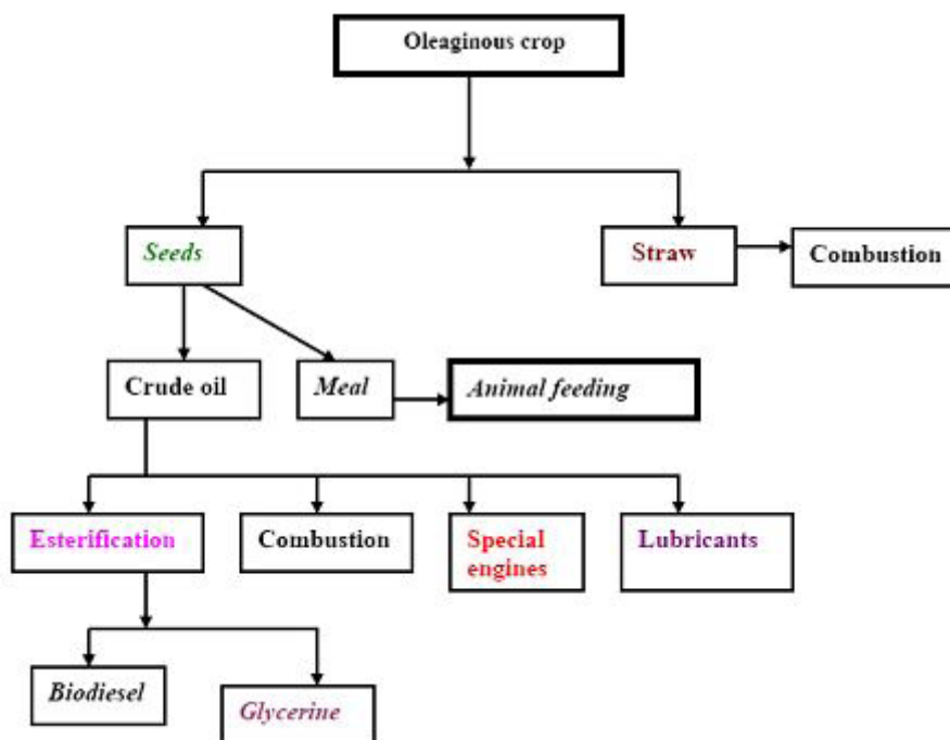
Figure 9: Flow chart of biodiesel production [12]
