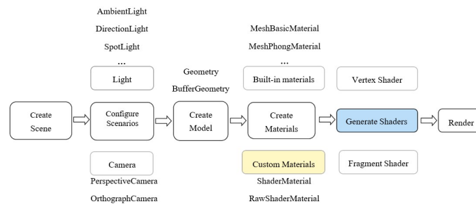
Figure 1: Three.js workflow diagram.
