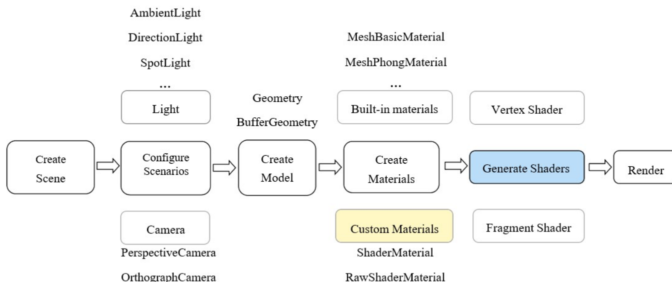
Figure 1: Three.js workflow diagram.
